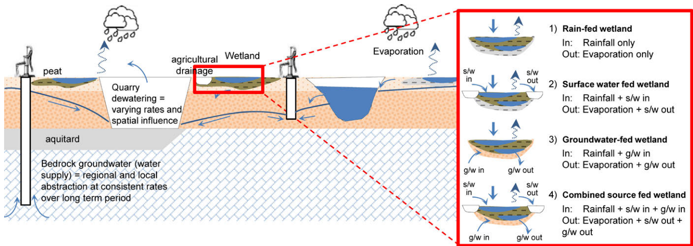
Figure 8 Rural hydrogeological influences.
